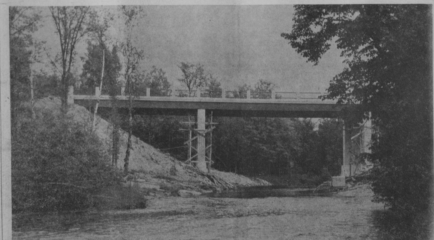
Pictured above is the new M-55 bridge over the East Branch of the AuGres river which is nearing completion. The structure is complete and the remainig work will be on the approaches. Constructed at a cost of $104,000 by the Construction Company, the new bridge is one of the most beautiful structures in the county. The structure replaces a narrow, one-lane bridge over the East Branch and the dangerous, steep approaches have been filled in.—HERALD PHOTO.
