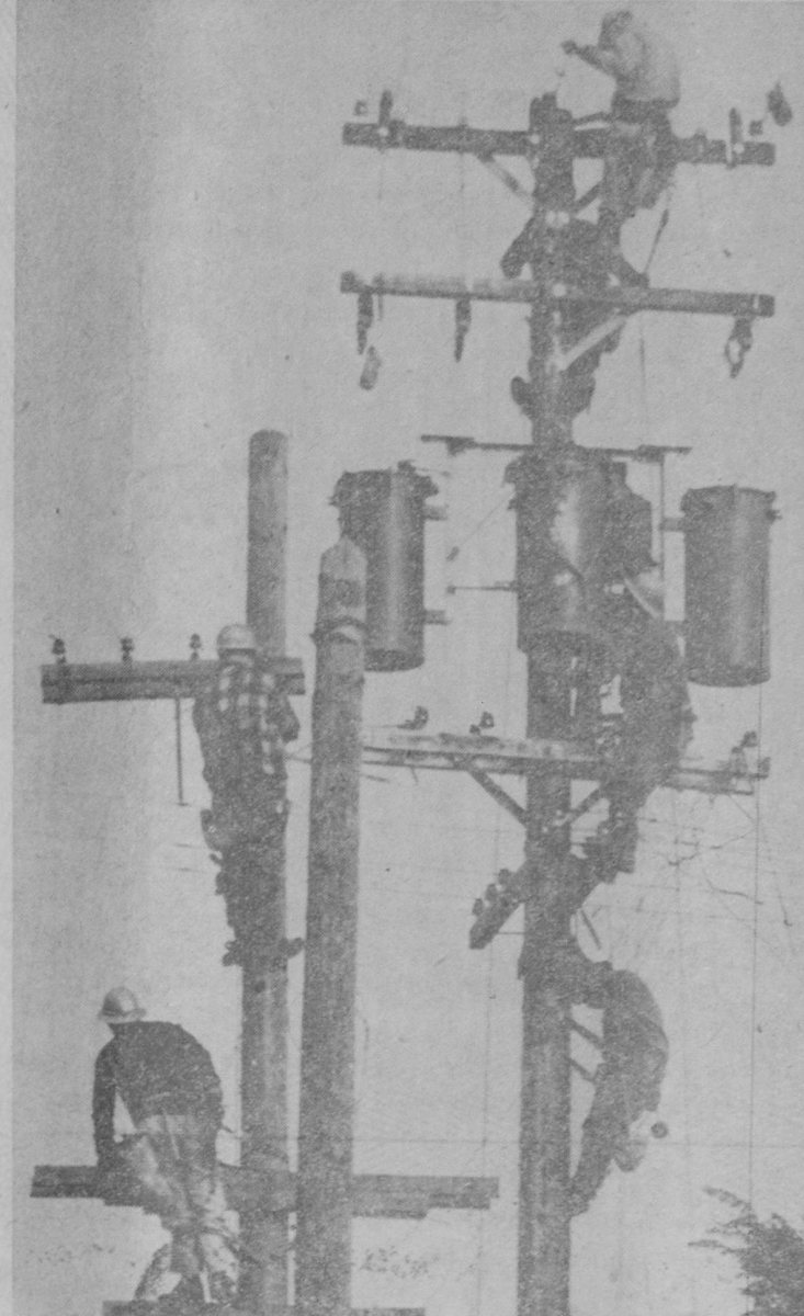
An unusual picture against the early morning sky—Consumers Power crew making a quick change-over of distribution lines to new transformer location last Sunday morning at Lake and First Streets.—Herald Photo.
