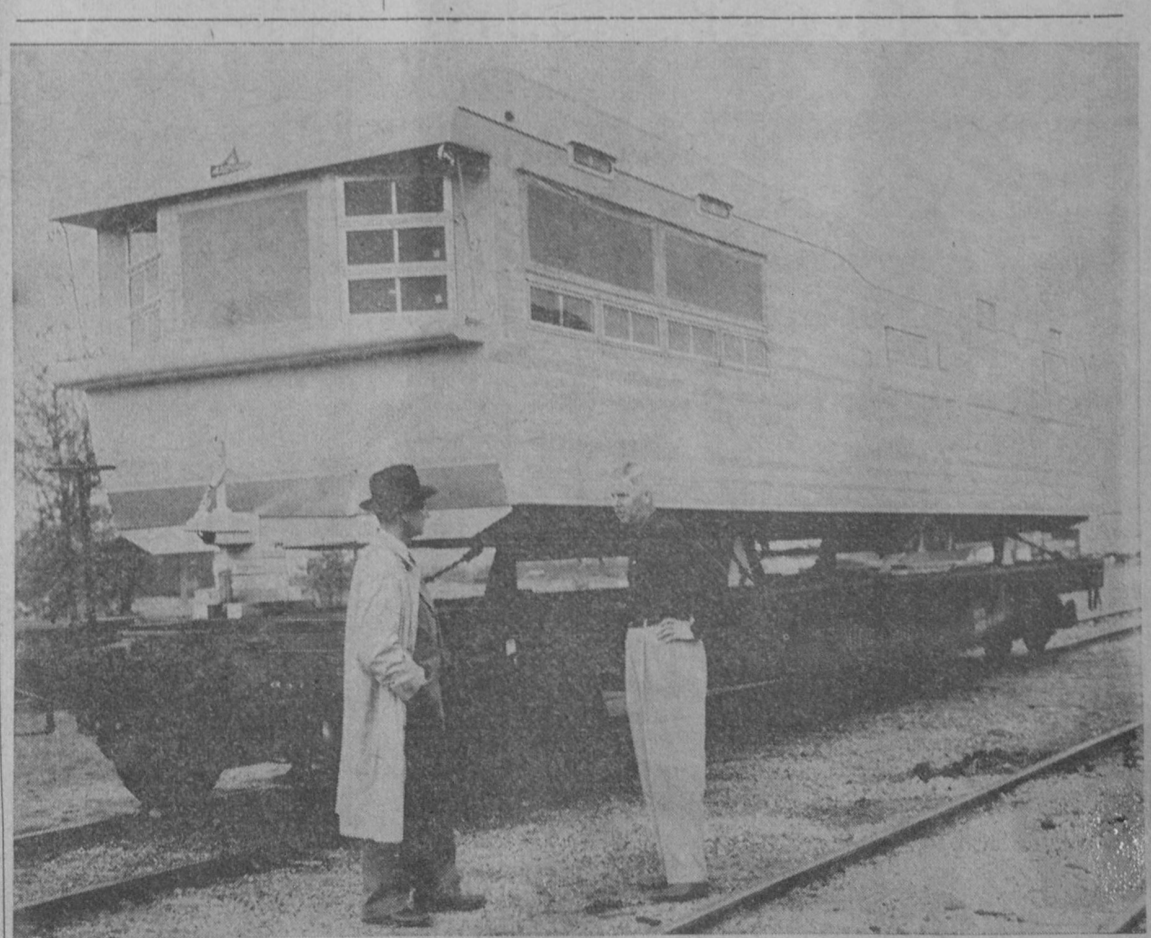
ANDERSON COACH COMPANY started a new system of shipping its 10-foot wide trailers to the western United States last Thursday afternoon when this rail car carrying a trailer manufactured at East Tawas left the Detroit and Mackinac yards here. Bound for Phoenix, Arizona, the trailer is the first to be shipped in this manner by Anderson Coach. Trailers are usually towed to their destination, but some states have laws preventing travel of a trailer this wide on state highways, and in some instances a flag man or trooper is required to assist in getting it through traffic. President of Anderson Coach Company, J. E. Jensen, right, and Charles A. Pinkerton, left, president and general manager of the Detroit and Mackinac Railway, are shown above inspecting the coach prior to its departure.—Tawas Herald Photo.
