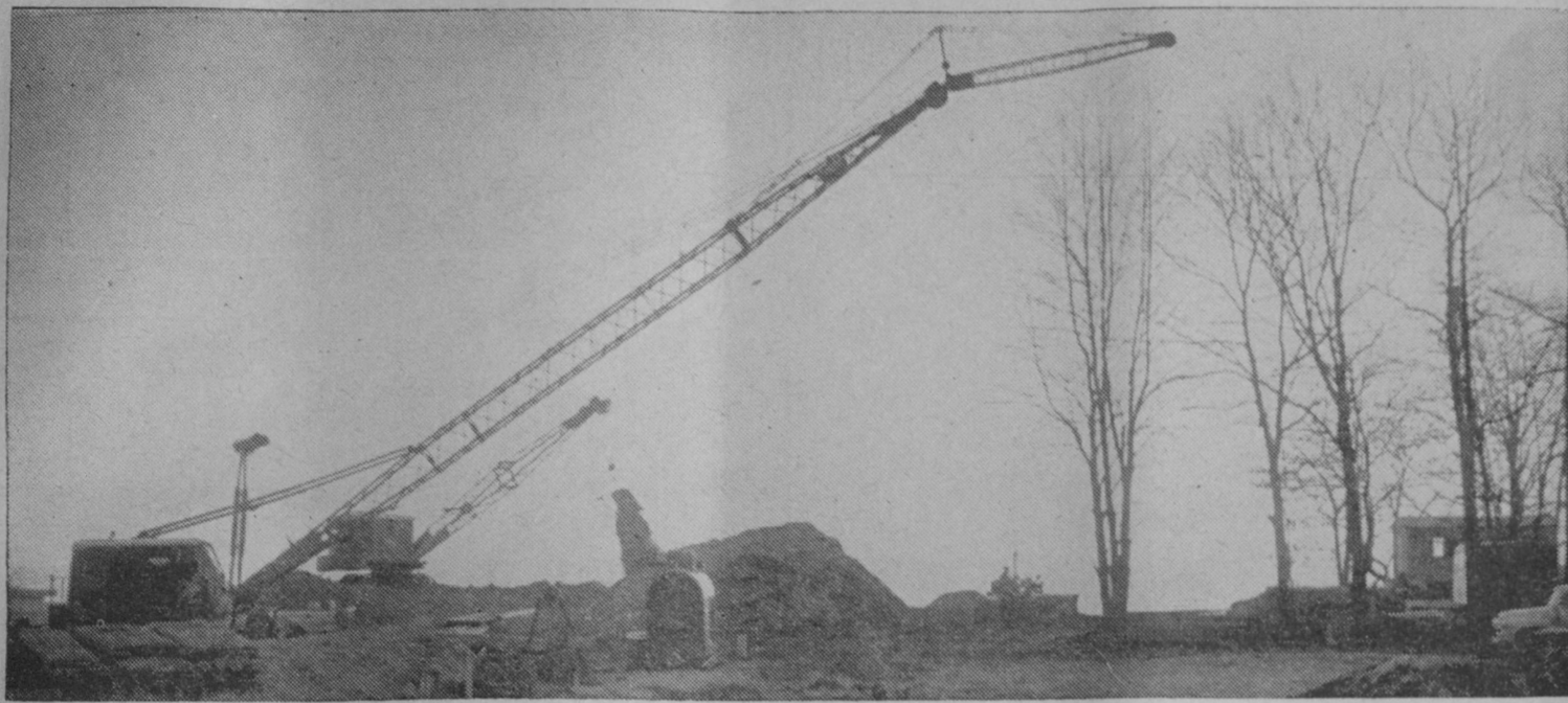
WORK ON PART of National Gypsum Company's new expansion program in Iosco County is pictured here. In the top photo heavy earth moving equipment is shown working at the site of the company's shore loading facilities south of Tawas City. In the photo at right a steam pile driver sinks stepped-top steel piling into the ground for footings at the site of the stockpile area west of the US-23 underpass. The pilings, driven deep into bedrock, are then filled under pressure with concrete. A conveyor system will carry gypsum rock from the stockpile area to the shore of Saginaw Bay and then over an enclosed gallery-type overhead conveyor system to ore carrier ships at a pier 375 feet from shore. Rock will be moved to the stockpile area from the company's new quarry on the Sand Lake-National City Road by the Detroit and Mackinac Railway Company.—Tawas Herald Photos.
