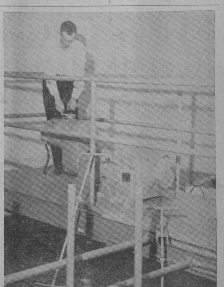
LEONARD GOSS, operator at East Tawas' new filtration plant, is shown above demonstrating controls of the plant's huge chlorinator equipment during open house Saturday.—Herald Photo.
