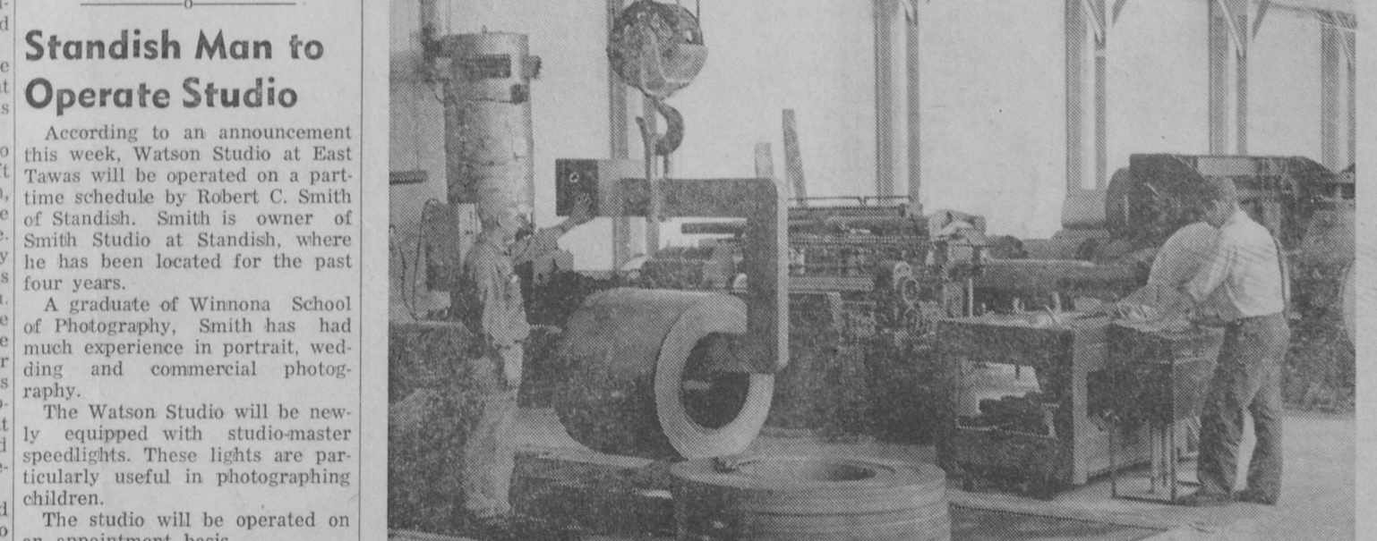
STEEL SLITTING machinery at Bopp-Busch Manufacturing Company plant at AuGres is shown in the above picture. The huge equipment takes rolls of steel in four-foot width and slits to requirements of the plant. It is the only such machine located north of Flint. (For additional pictures, please turn to page 8.)—Tawas Herald Photo.
