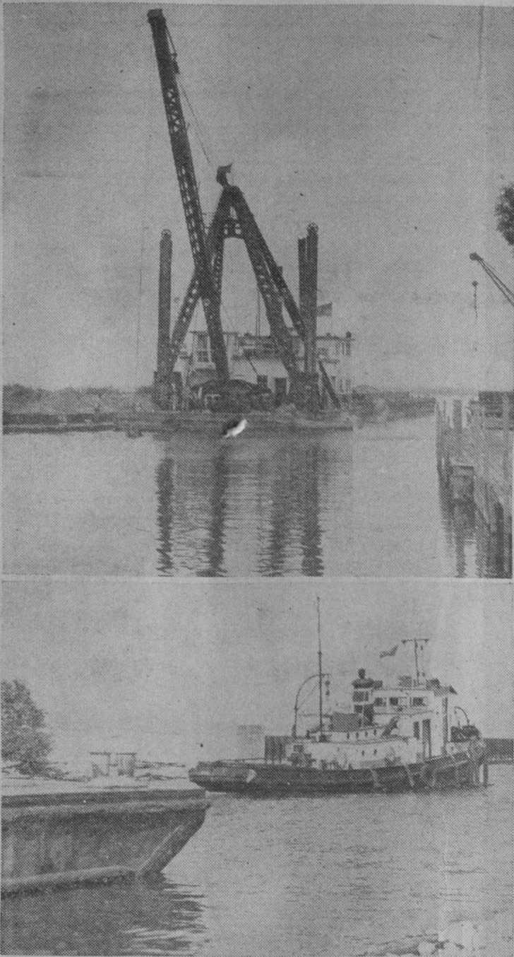
DREDGING OPERATIONS at the mouth of the AuSable River on Lake Huron have been under way for the past two weeks. These two pictures show activities last Wednesday. Work is being performed by the United States Army Corps of Engineers. The top picture shows the huge dredging equipment, while the picture at bottom shows a tugboat with a scow in tow as it heads out to the Lake Huron dumping grounds.—Tawas Herald Photos.
