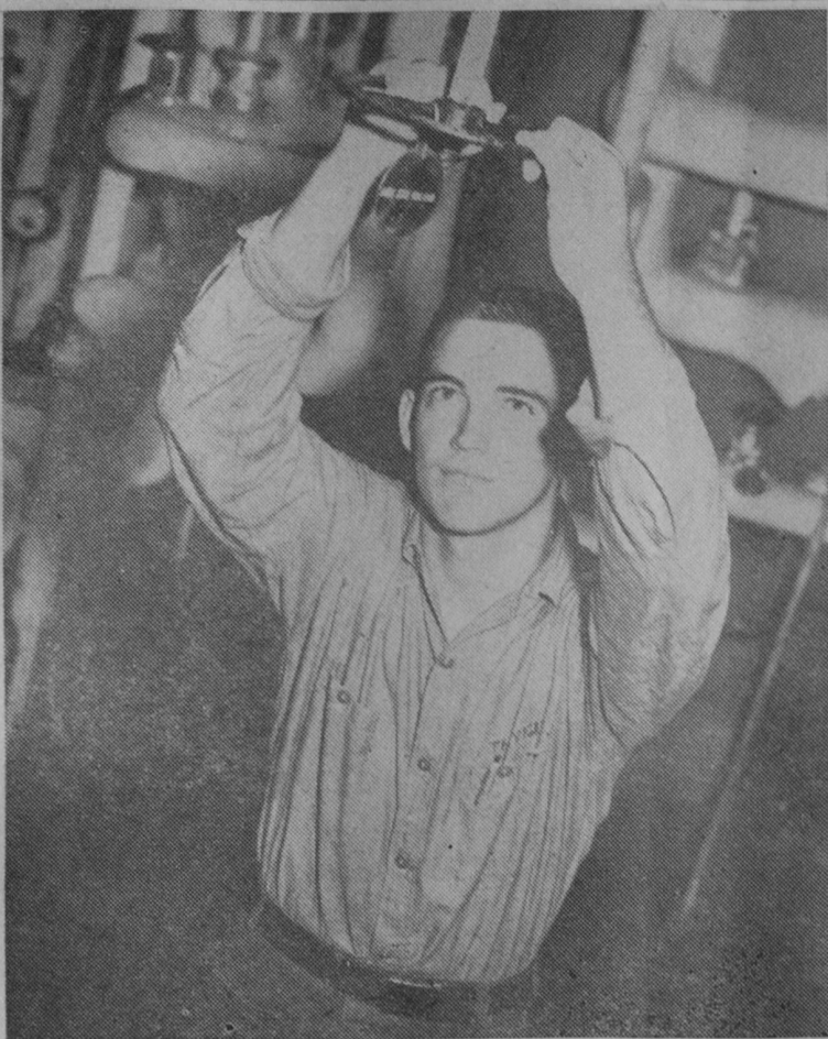
LEONARD A. THAYER —fireman apprentice, USN, of Long Lake, closes the dumping valve to the auxiliary exhaust steam line during a 12-week course of instruction at the Machinist's Mate Class "A" School at United States Naval Training Center, Great Lakes, Illinois. This valve prevents the overloading of steam on a ship's steam engines by allowing the steam to be exhausted when pressure builds too high. It is only one of many technical phases of instruction undergone by students at the school.
