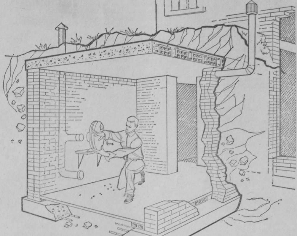
DUAL-PURPOSE underground fallout shelter of clay masonry construction and designed to be built as part of new house would combine some of the best features of the Defense Department's new "Family Shelter Designs" handbook available at state and local civil defense offices.
