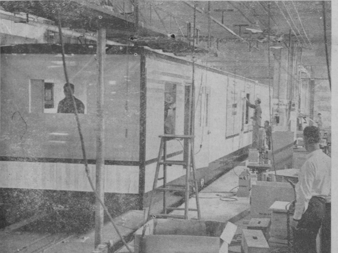
PRODUCTION LINE at Anderson Coach Company's Baldwin Township plant is pictured here. Standing at right is Orville Stiehl, general manager. Two coaches were going through the line when this picture was snapped last week.—Tawas Herald Photos.
