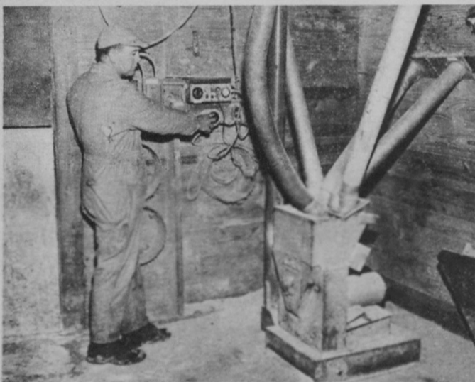
Using his mix mill operation in his barn, the dairy feed is made once a week and augered directly to a special bin near the milking parlor.
