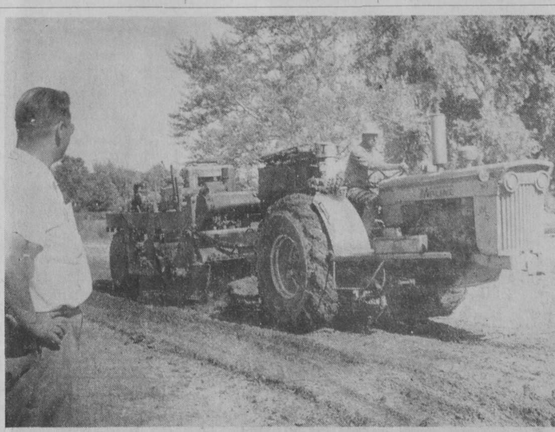
CONSTRUCTION on streets in Tawas City and East Tawas is being completed this week by Yockey Construction Company, Alpena. Watching this large piece of machinery as it prepares a soil base stabilized with asphalt on First Street, Tawas City, is James Yockey, one of the owners of the Alpena paving firm.—Tawas Herald Photo.
