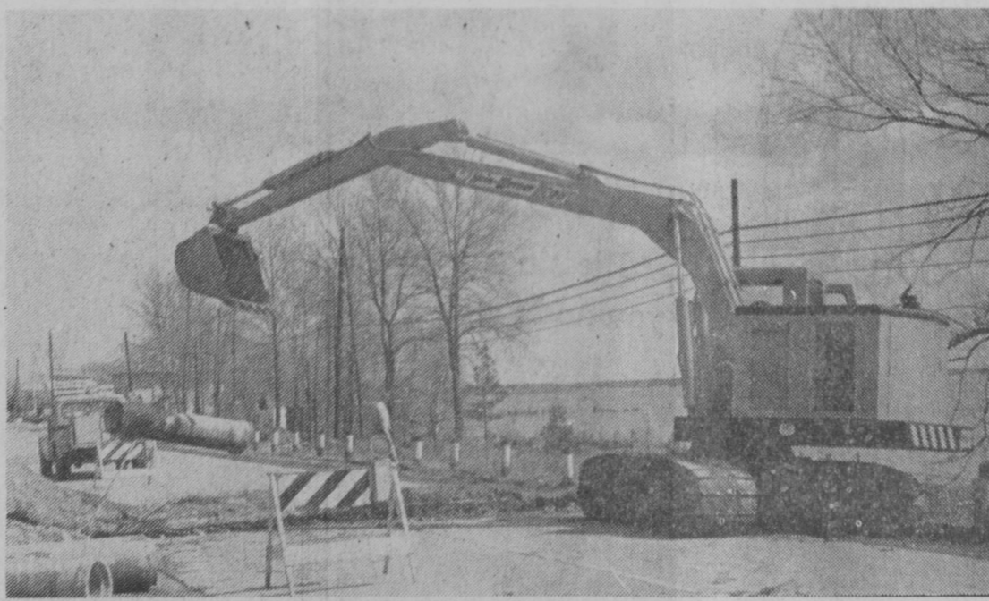
COMPLETION of the modernizing of US-23 in Isosco County was completed during 1966. Heavy equipment used in constructing the final link through Tawas, completed with only minor interruption of traffic, is pictured above along the bay shore.—Tawas Herald Photo.
