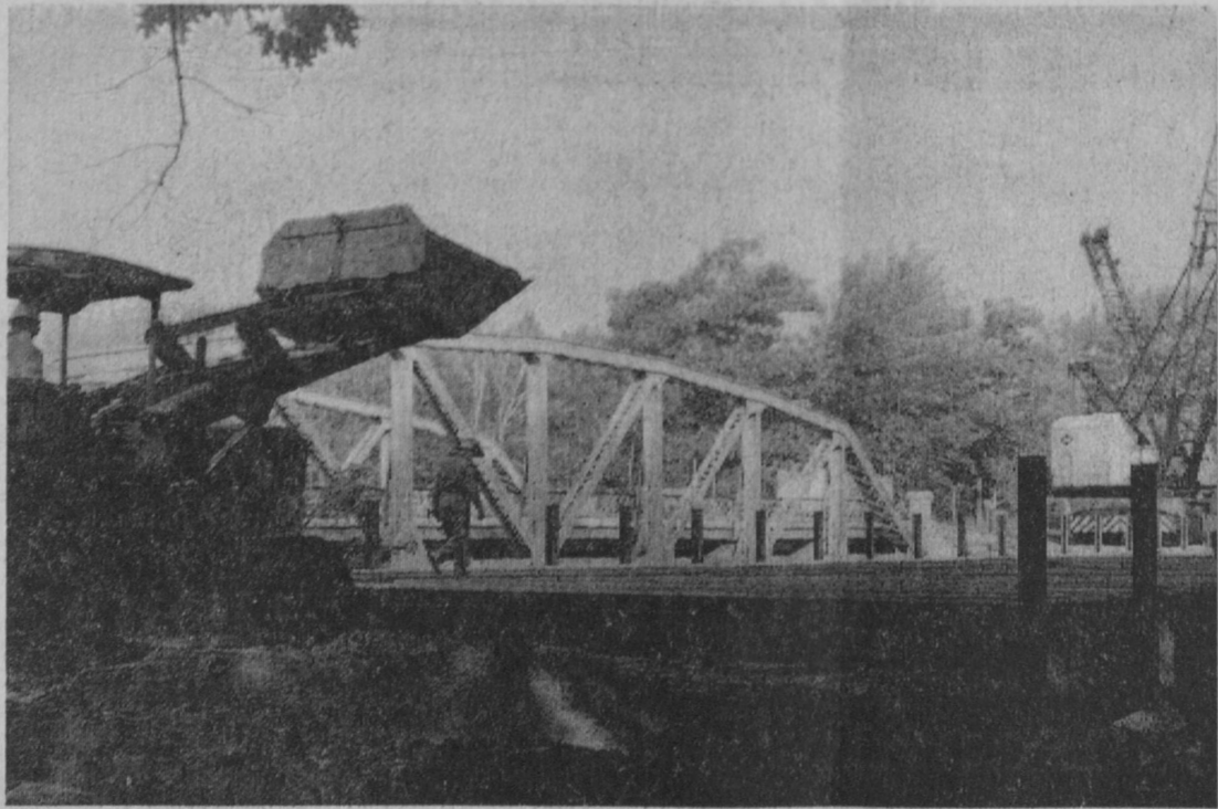
WORK IS UNDER WAY on constructing a temporary span over the Whitney Drain on US-23 south of Tawas City which will carry traffic while a new bridge is being constructed to replace the old "Singing Bridge." This is one of several old steel bridges which are being replaced by the Michigan Department of State Highways. Another bridge being replaced is one over the AuSable River at Oscoda. A new Mill Street bridge, which will carry US-23 traffic while the downstream bridge is being constructed, was opened last week.—Tawas Herald Photo.
