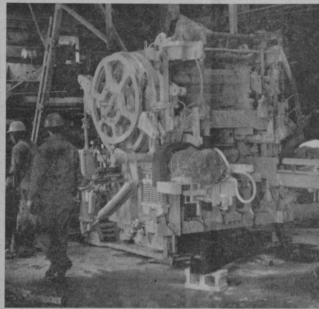
A NEW concrete block machine manufactured by Besser Manufacturing Company, Alpena, is being installed at Huron Building Supplies, Tawas City. The new 20-ton unit replaces a machine which was purchased about 15 years ago. The new machine is
