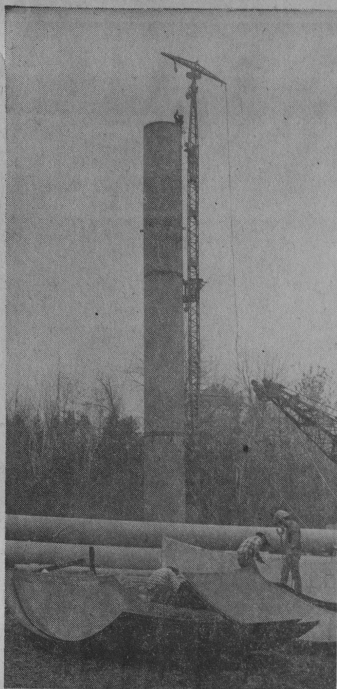
WORK STARTED MONDAY on erection of a 500,000-gallon overhead water storage tank at the industrial park in Tawas City as part of the area's water expansion program. Workmen of Pittsburgh-Des Moines Steel Company are shown Tuesday afternoon preparing to hoist another prefabricated section in place to form the central column. Workmen in the foreground are preparing other sections of the tank for installation.—Tawas Herald Photo.
