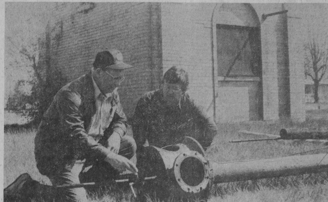
INSPECTING the top section of a six-inch casing removed from Tawas City's standby well are City Mgr. Reginald Bublitz, left, and Theodore (Ted) St. James, electrician. The more than 40-year-old well became inoperable Thursday and a new submersible pump was to have been installed Tuesday.—Tawas Herald Photo.
